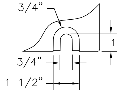
SLOT PLAN
